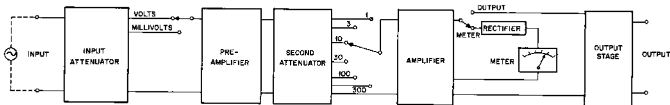
BLOCK DIAGRAM
